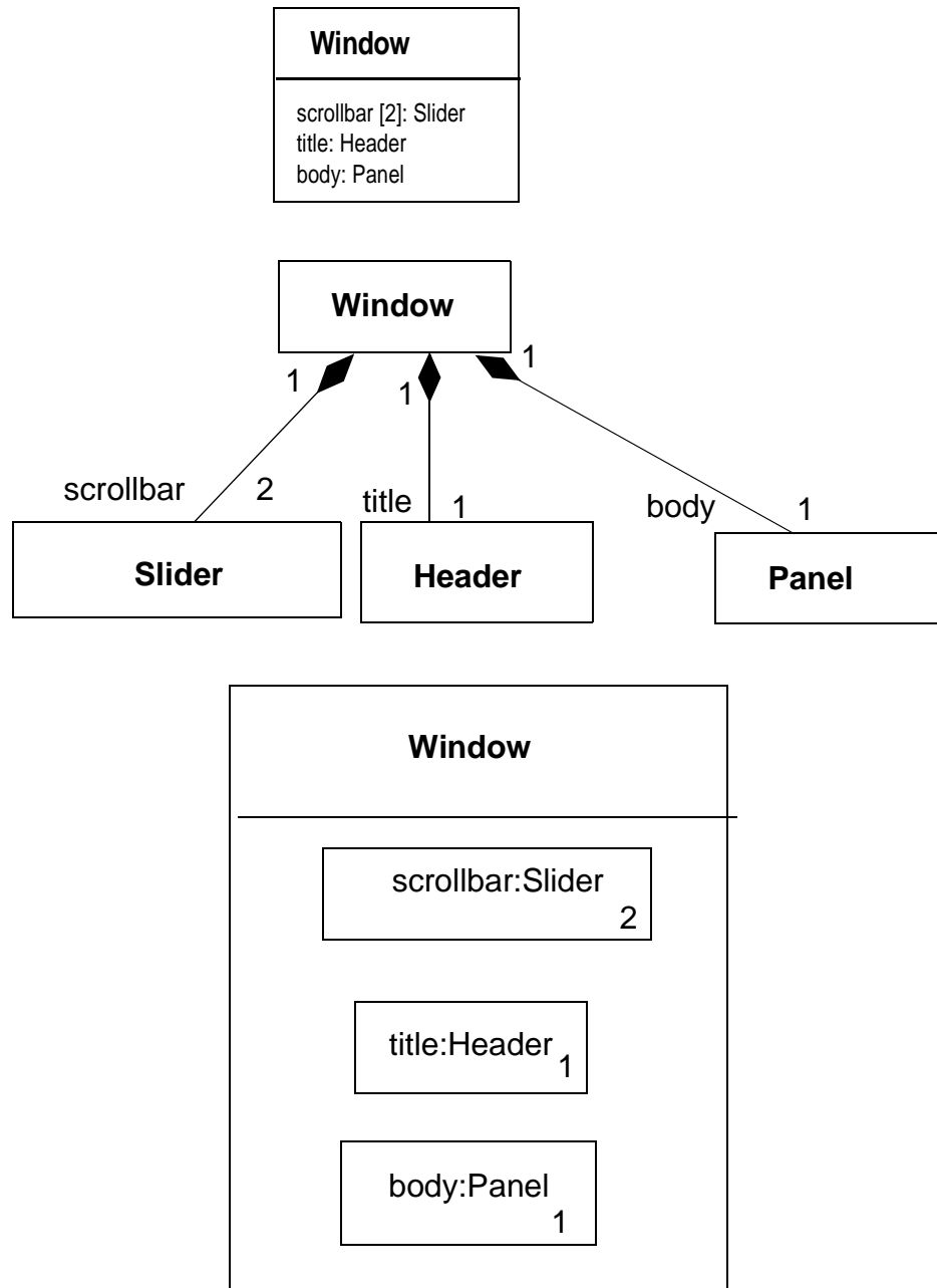
Figure 3-36 Different Ways to Show Composition
