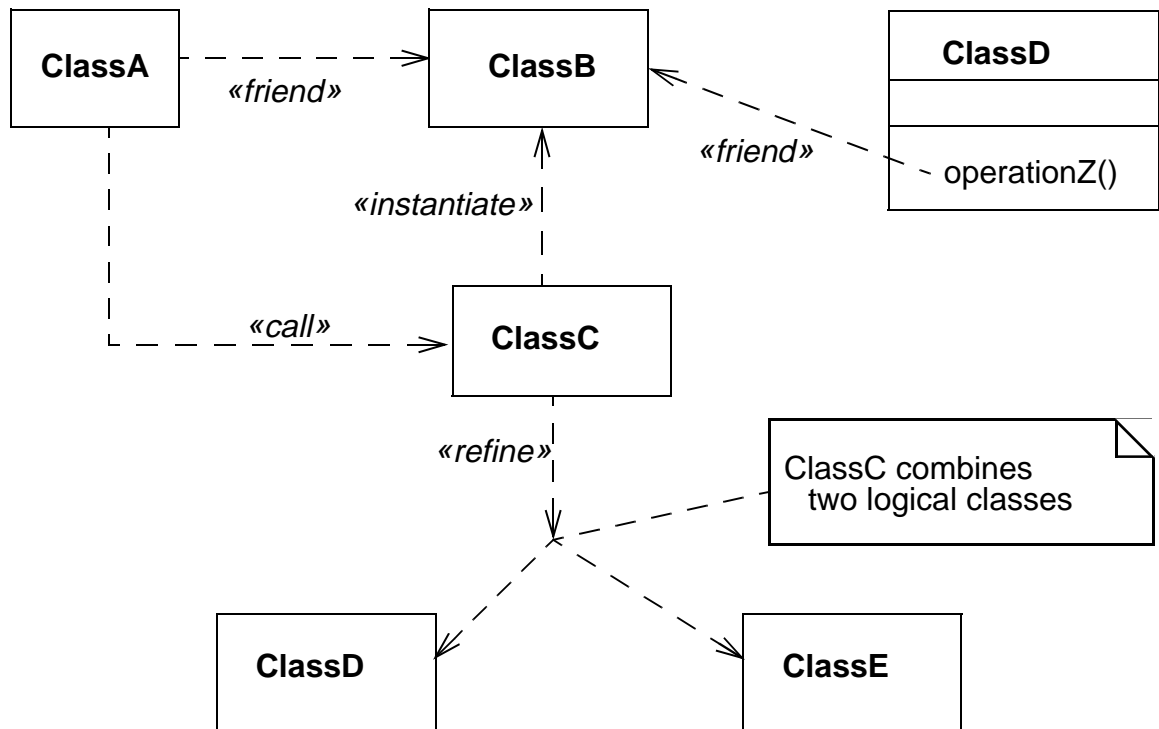
Figure 3-41 Various Dependencies Among Classes
