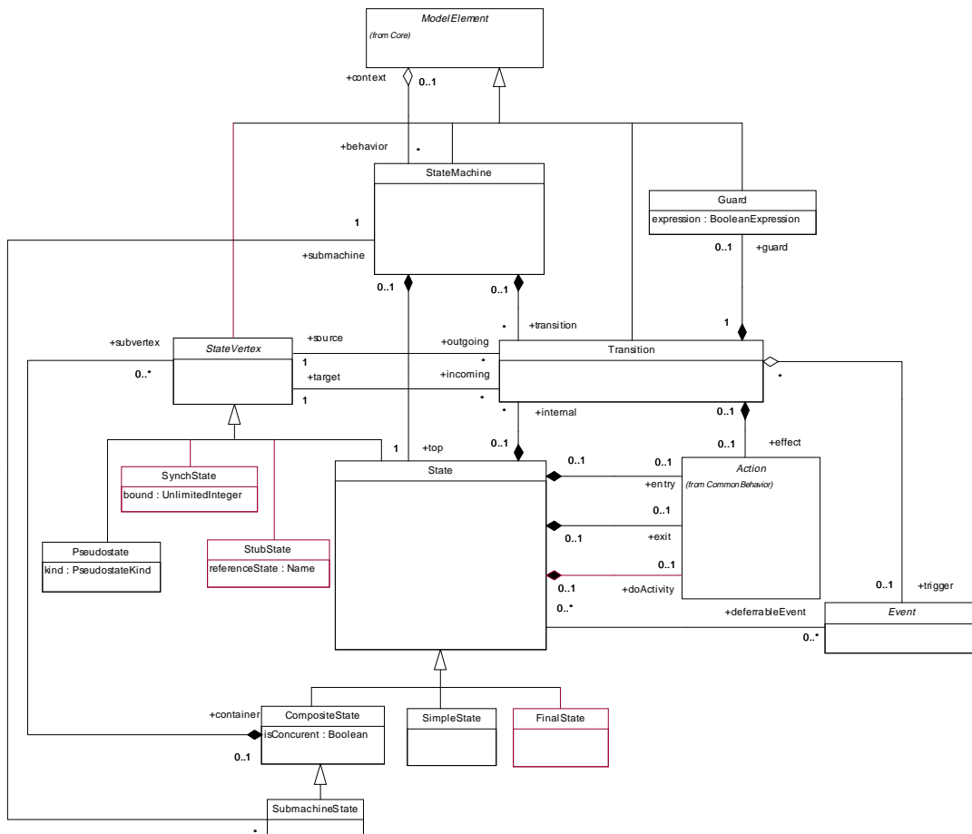
Figure 2-21 State Machines - Main
