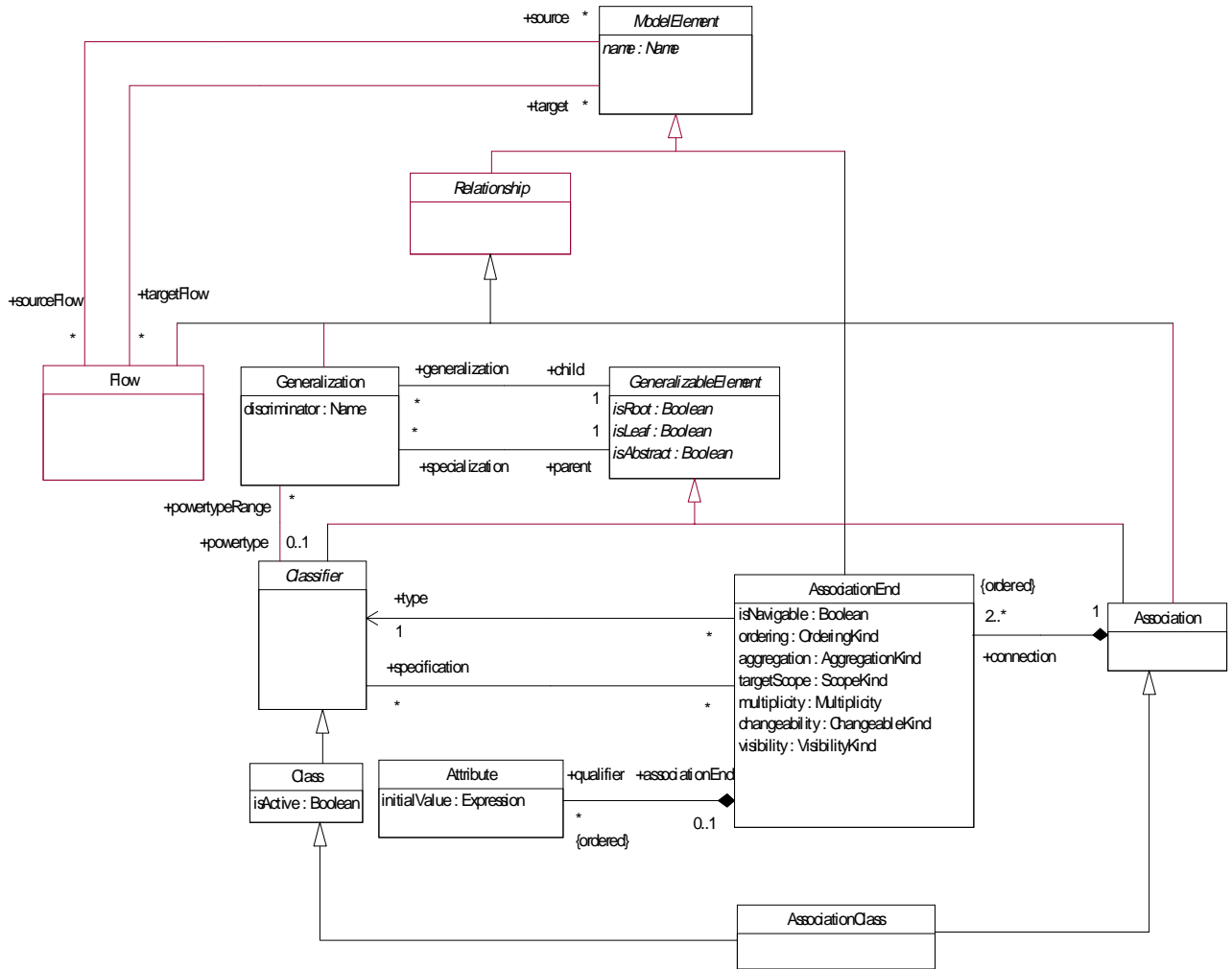
Figure 2-6 Core Package - Relationships
