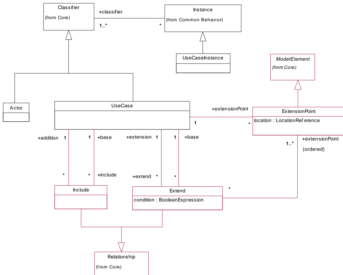
Figure 2-18 Use Cases
