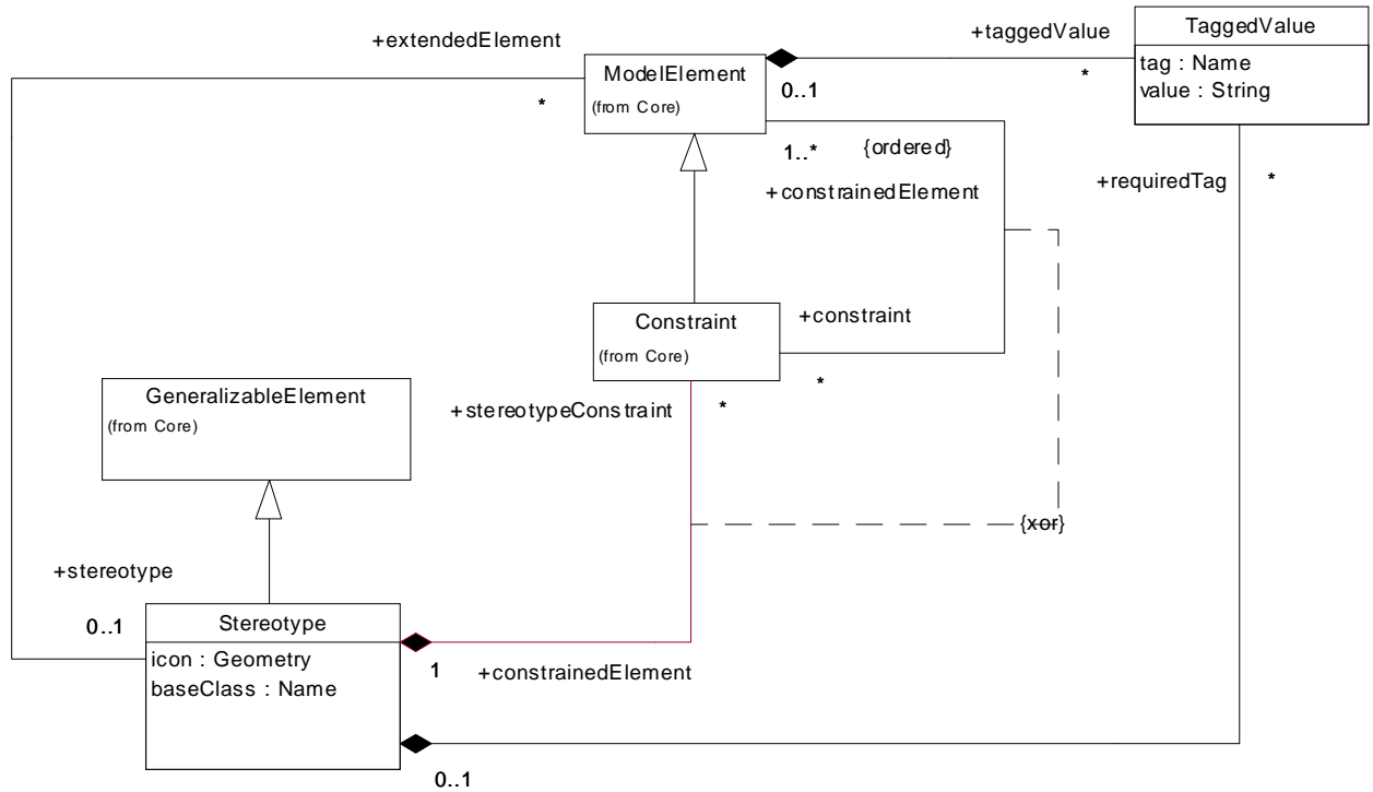
Figure 2-10 Extension Mechanisms
