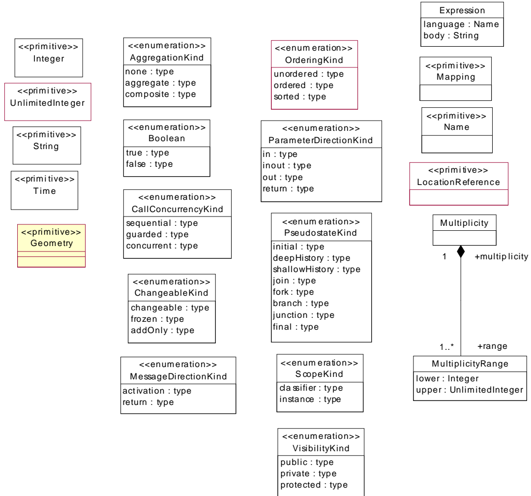
Figure 6-6 Data Types
