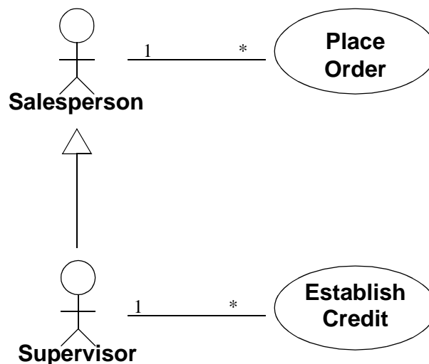
Figure 3-46 Actor Relationships
