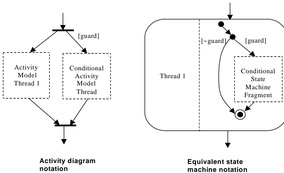
Figure 2-28 State machine meaning for activity diagram
