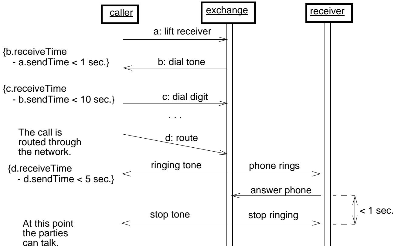
Figure 3-47 Simple Sequence Diagram with Concurrent Objects (denoted by boxes with thick borders).
