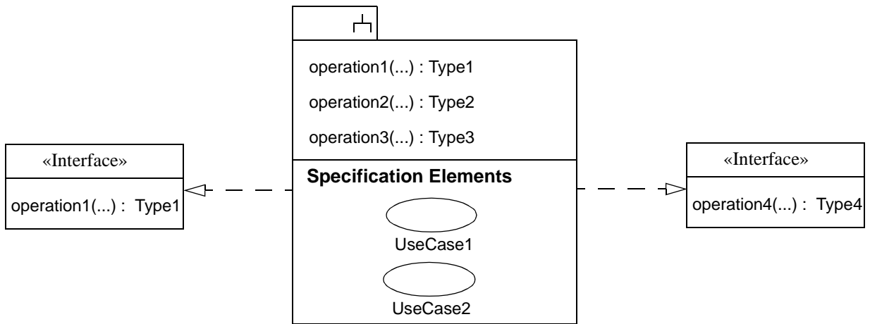
Figure 3-10 First schematic example where the specification/realization distinction is explicit
