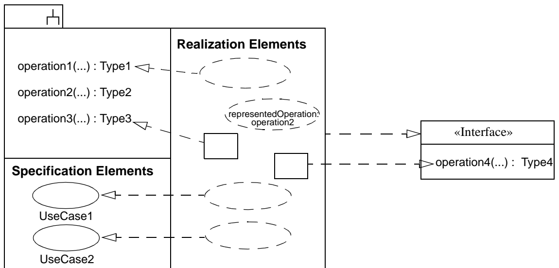
Figure 3-12 Third schematic example where the specification/realization distinction is explicit
