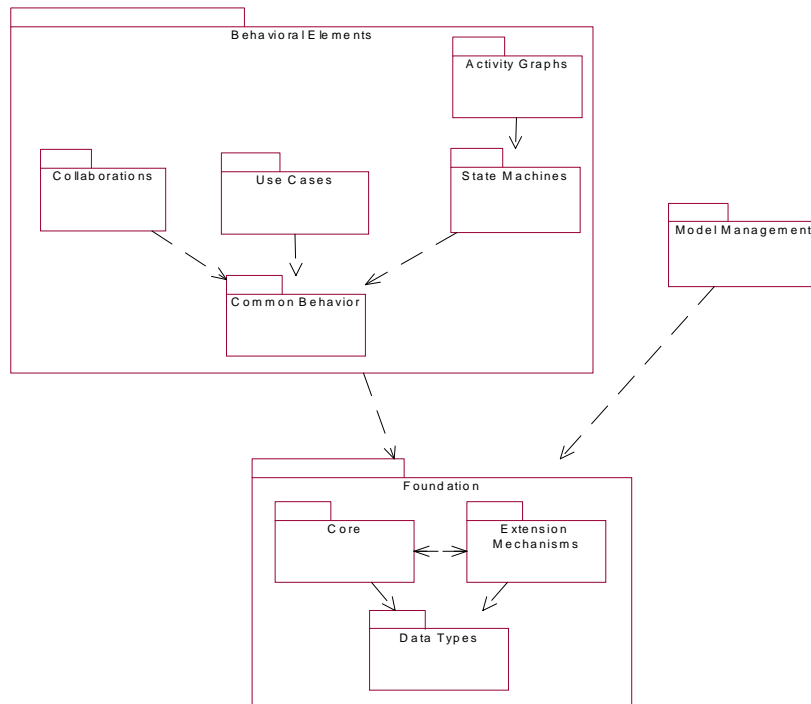
UML Class Diagram Showing Package Structure
