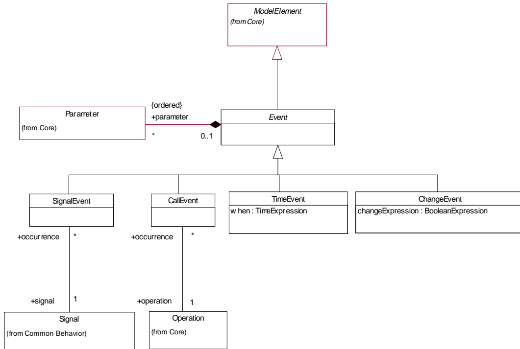
Figure 2-22 State Machines - Events
