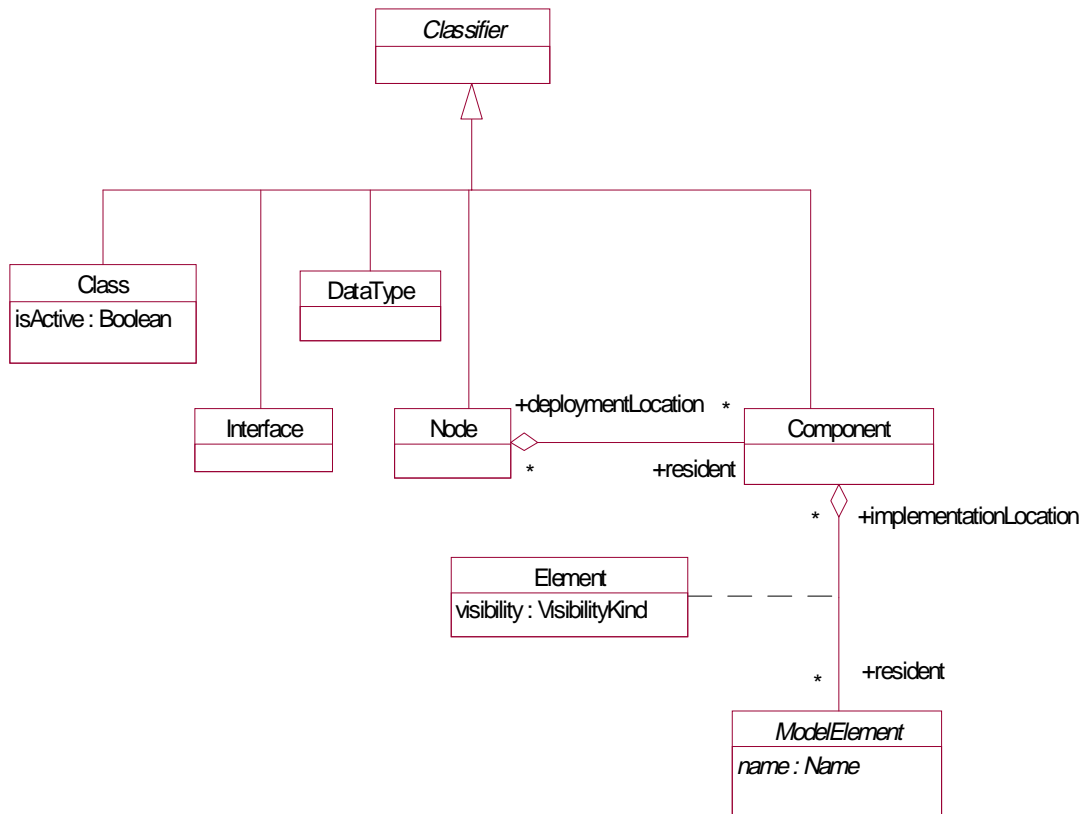
Figure 2-8 Core Package - Classifiers
