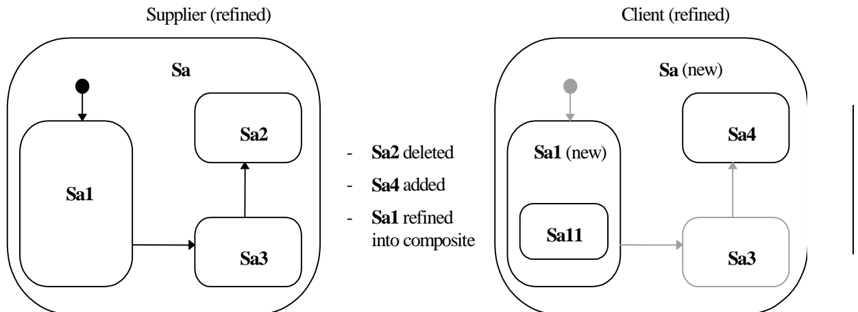
Figure 2-26 State Machine Refinement Example
