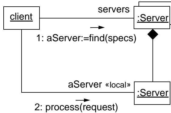
Figure 3-57 Multiobject
