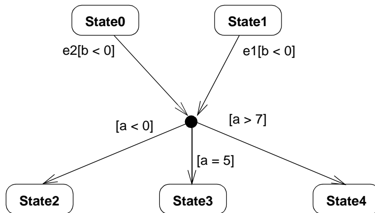
Figure 3-68 Junction points
