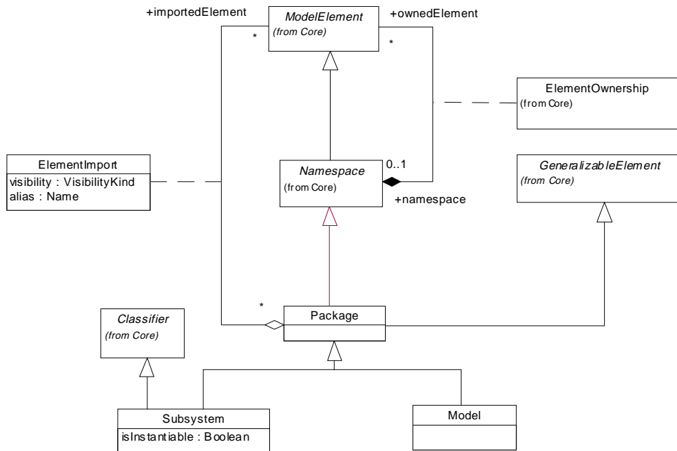
Figure 2-29 Model Management
