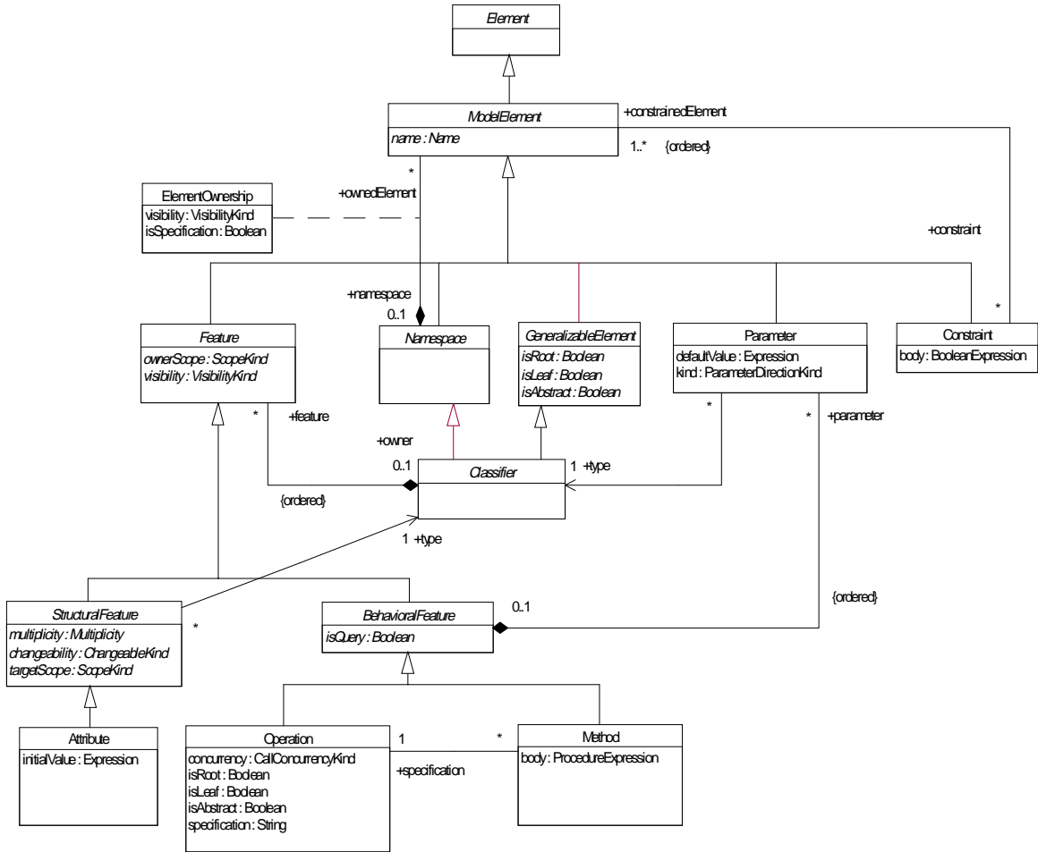
Figure 2-5 Core Package - Backbone
