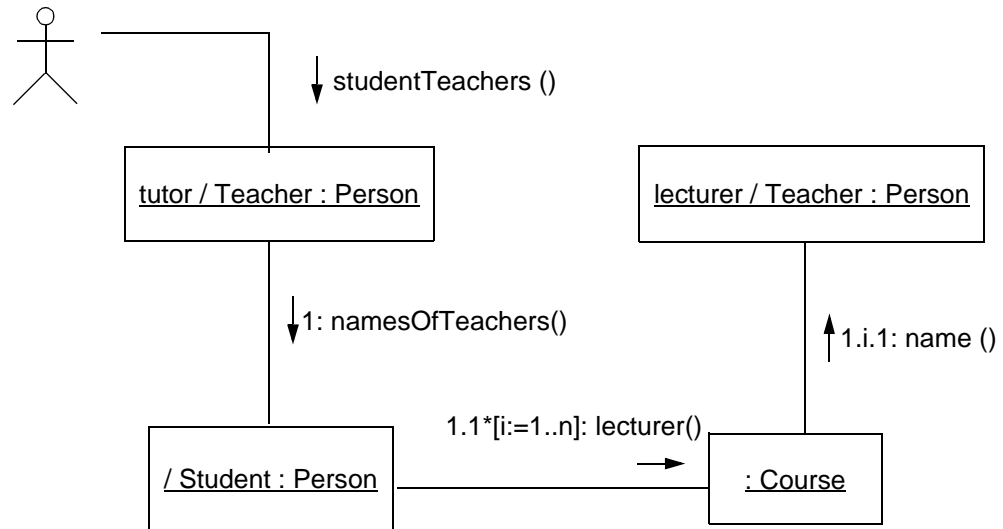
Figure 3-52 Collaboration Diagram at instance level in which some of the Objects play the same role. The instances conform to the Collaboration shown in Figure 3-51 on page 3-109.
